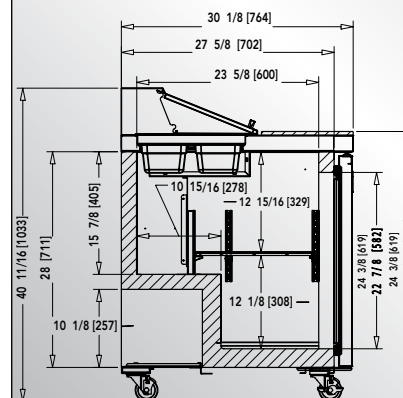
Vista lateral / Side view: Pulg. [mm] / In [mm]:
