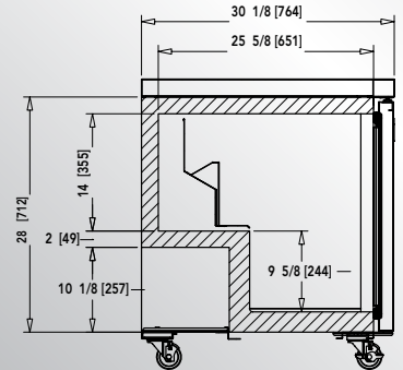
Vista lateral / Side view: Pulg. [mm] / In [mm]:
