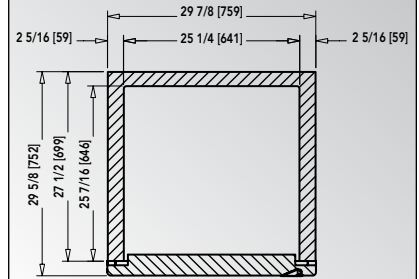
Vista superior / Top view: Pulg. [mm] / In [mm]:
